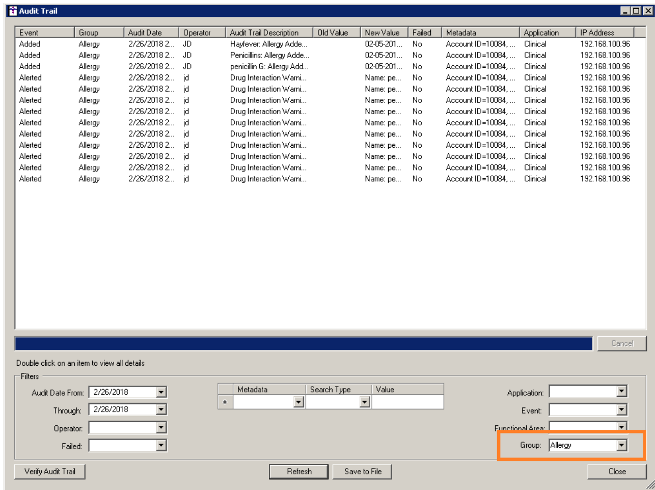
Figure 1 – Audit Trail
