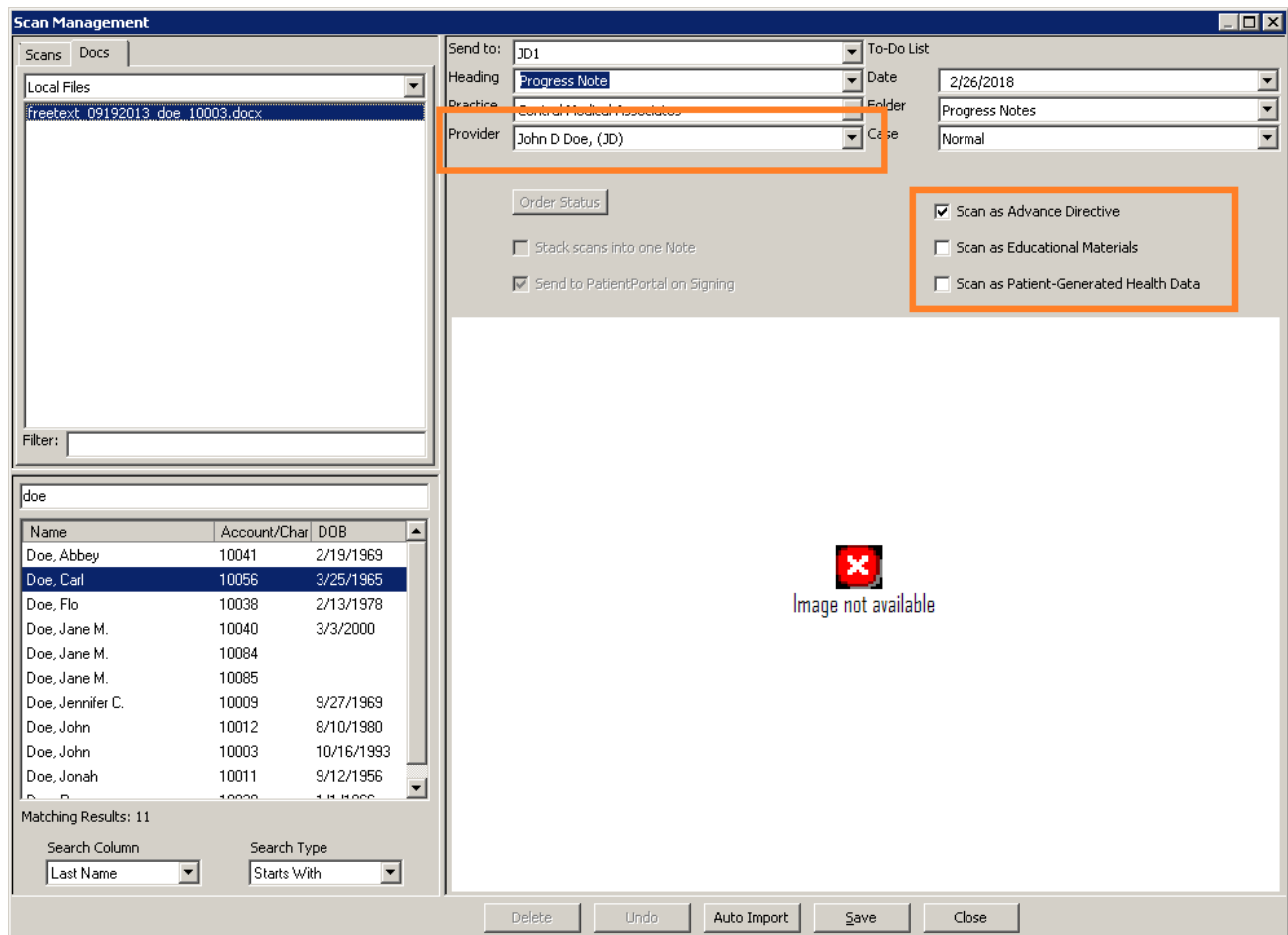
Figure 4 – Scan Management
