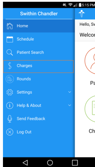
Figure 3 – Mobile Menu
