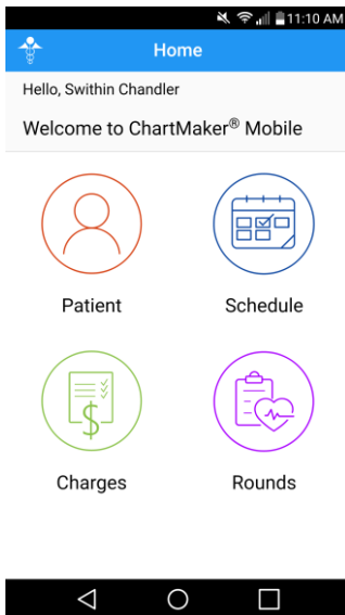
Figure 2 – Home
