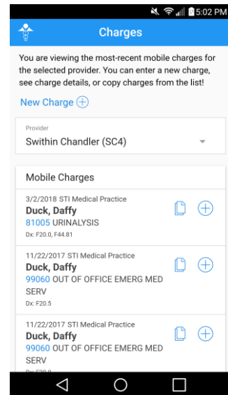
Figure 4 – Charges
