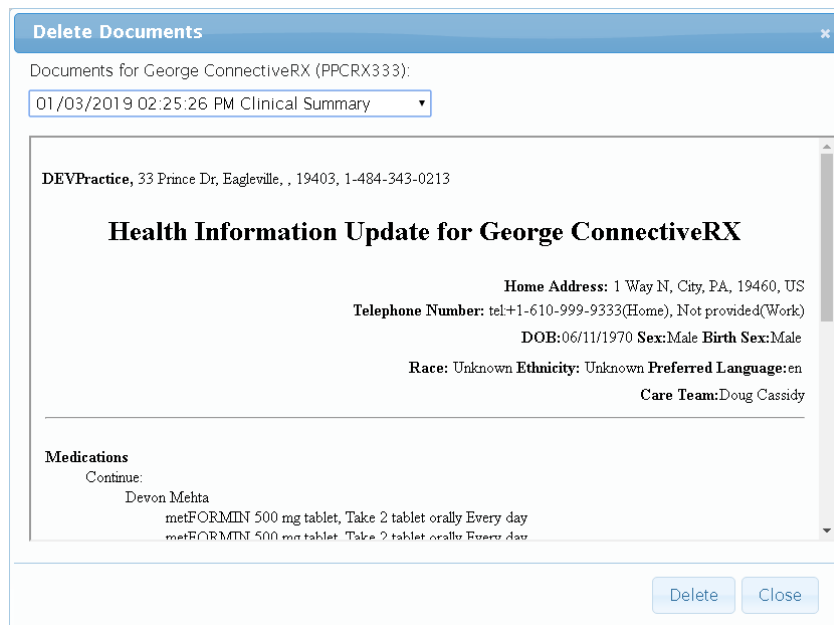
Figure 2 – Delete Documents
